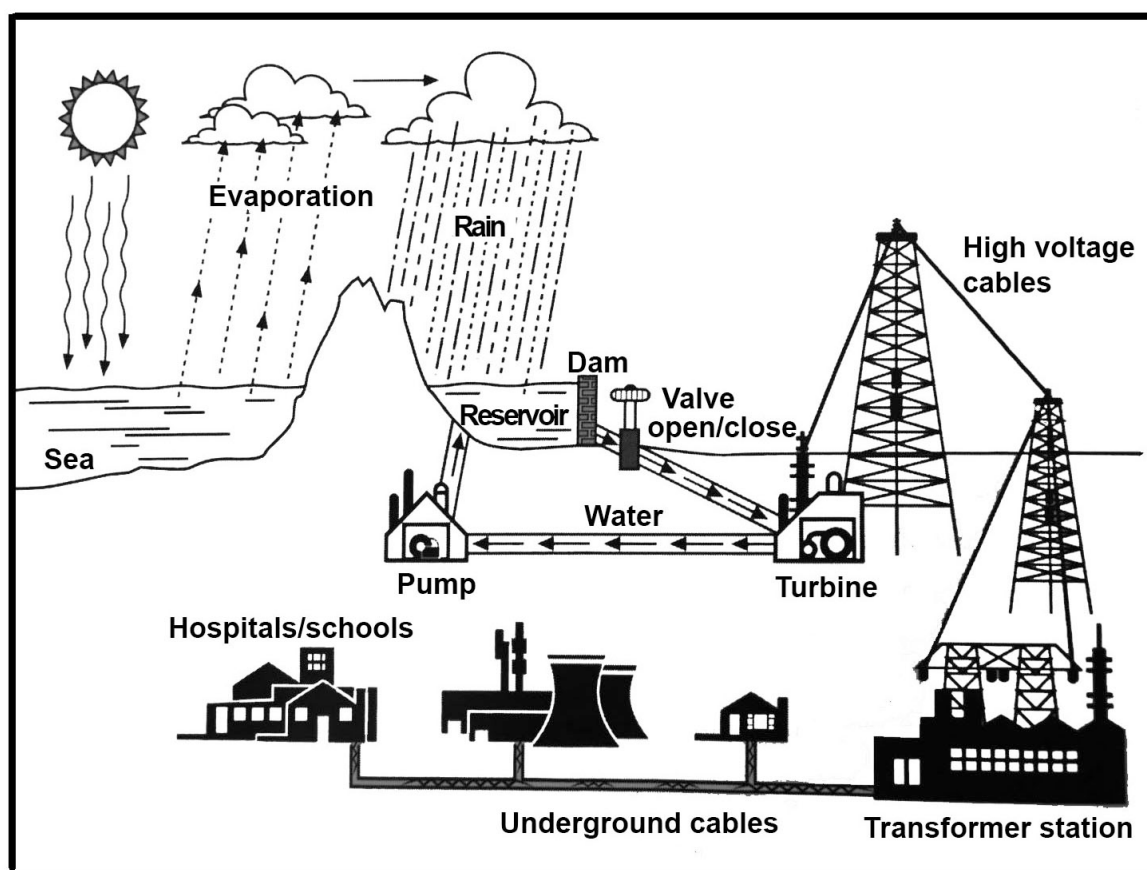
Hydro-electric power generation
